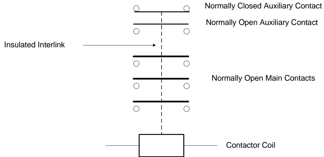
Layout of a 3 Pole Contactor
