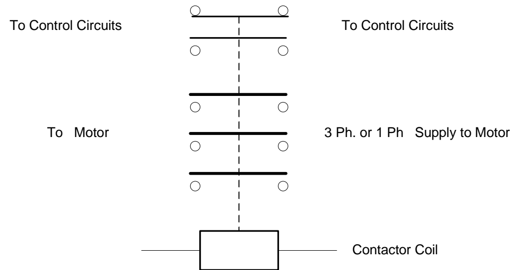
Contactor connections
