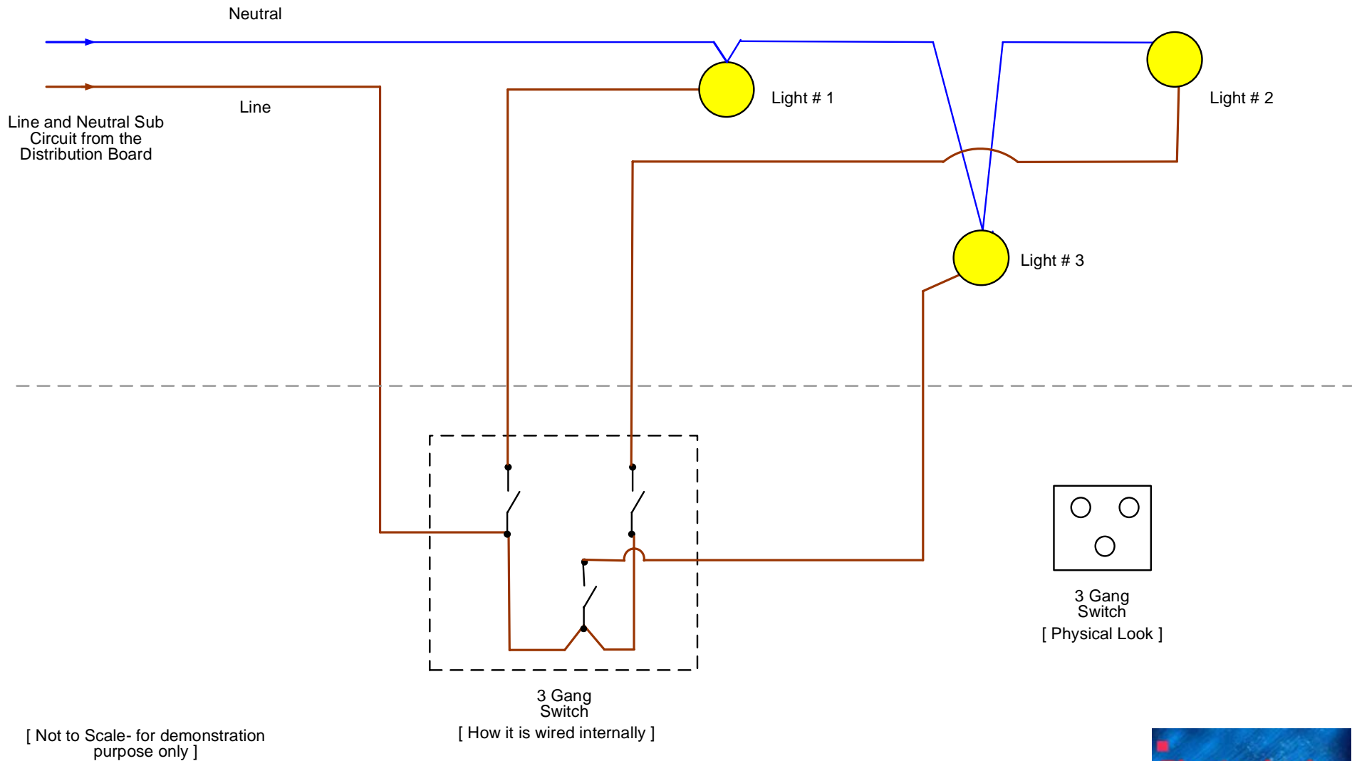
An example of how one sub circuit is used for wiring several light points
